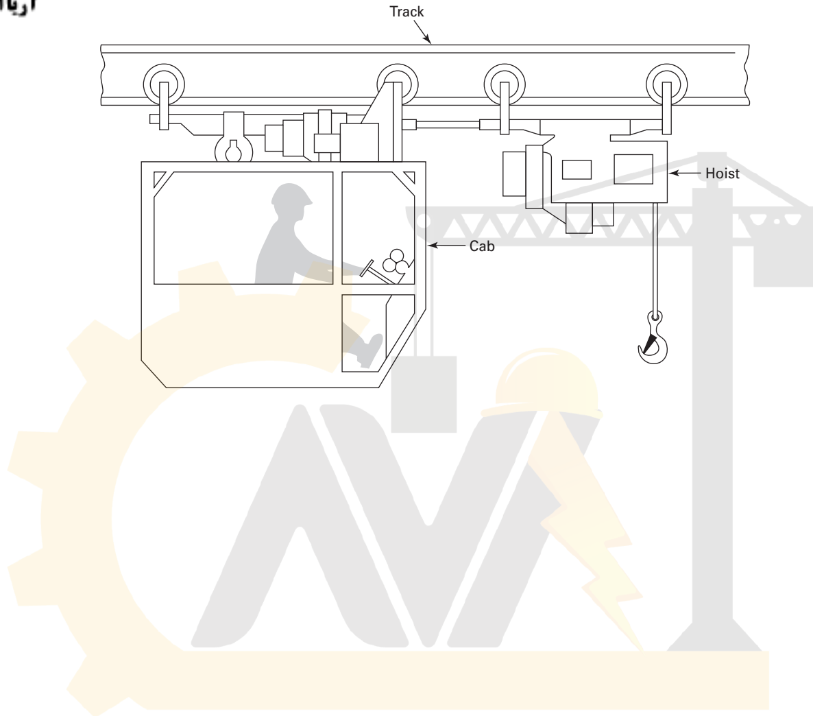
Fig. 17-0.2-13 Cab-Operated Trolley
