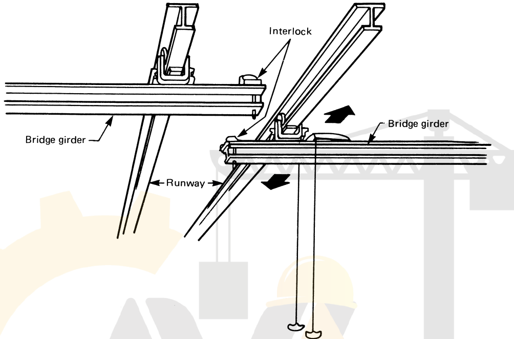
Fig. 17-0.2-11 Interlocking System for Underhung Crane
