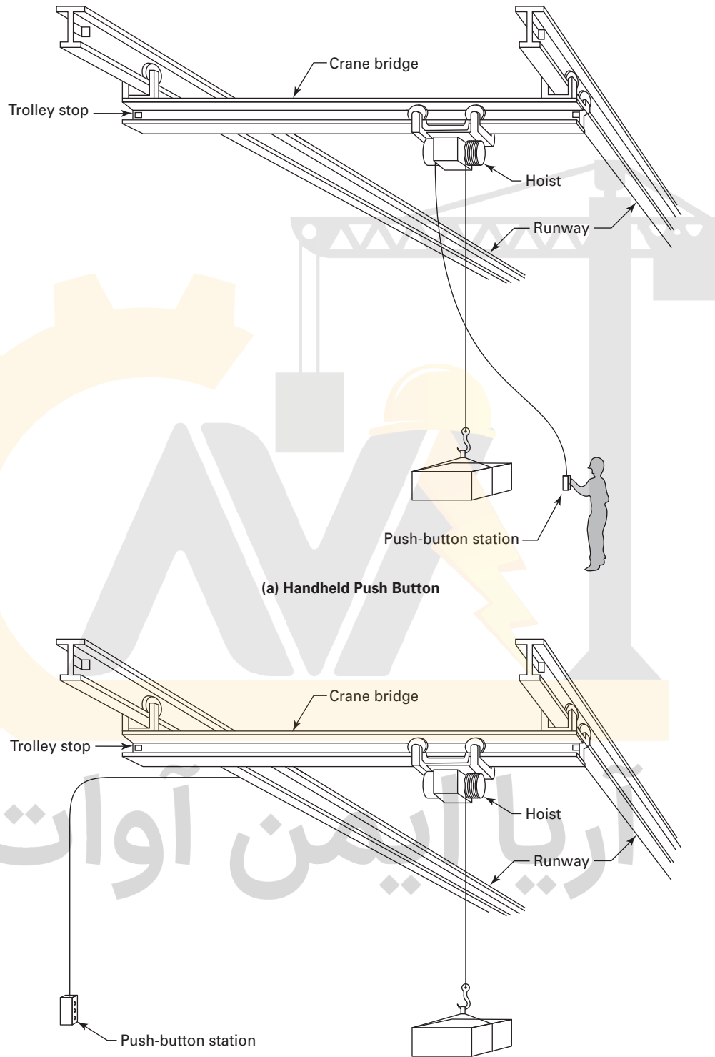
(b) Wall-Mounted Push Button
