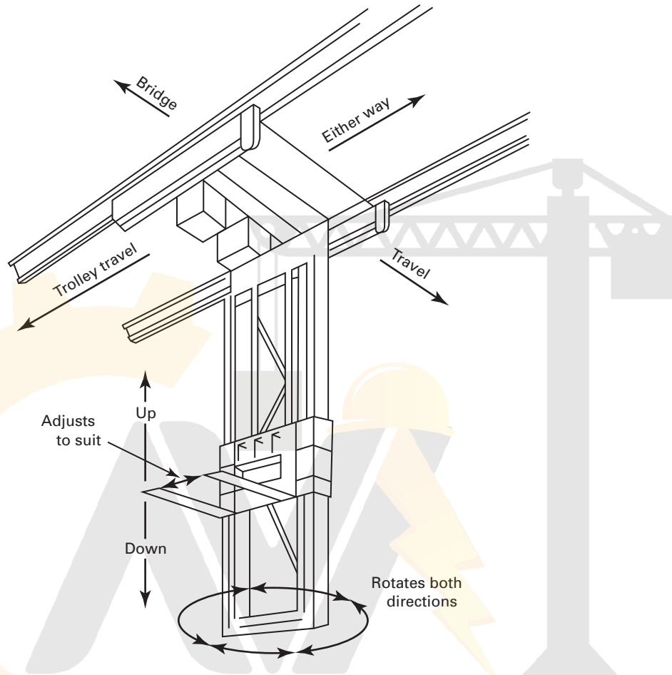
Fig. 18-0.2.1-3 Underhung Stacker Crane Movement
