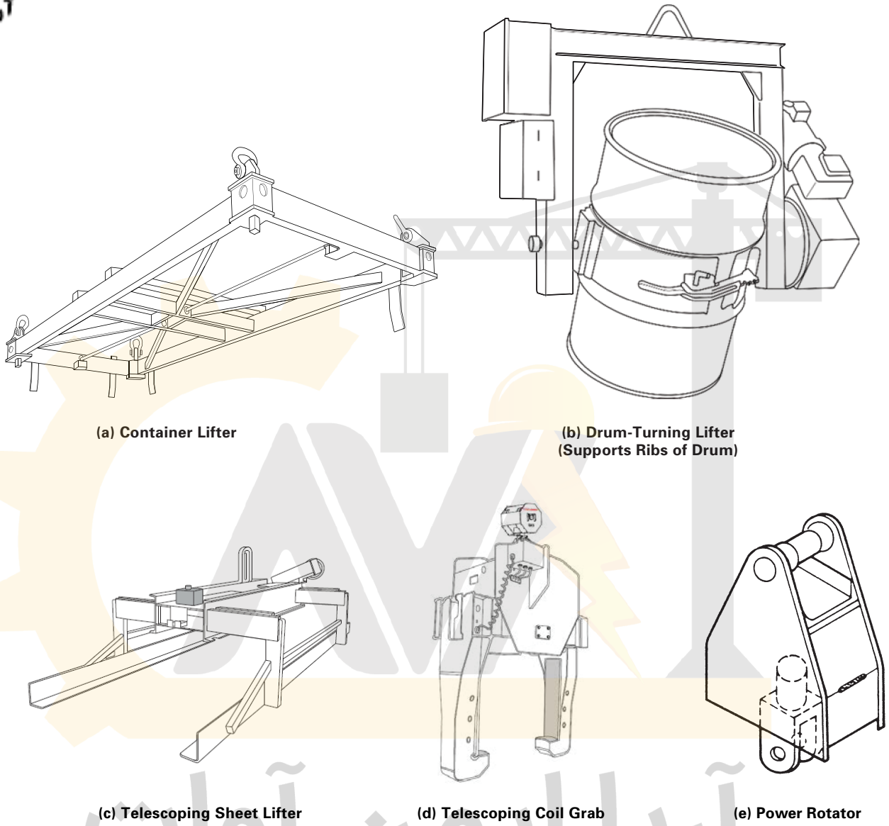
Figure 20-1.1-2 Mechanical Lifters
