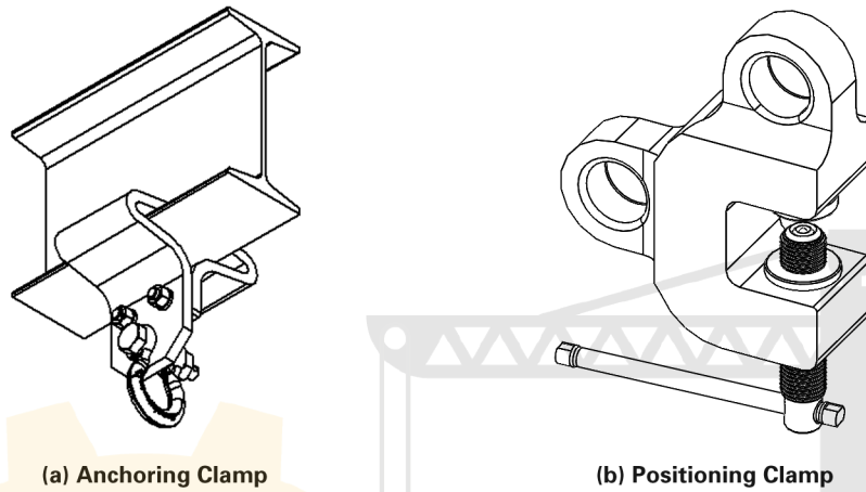
Figure 20-6.0-4 Anchoring and Positioning Clamps
