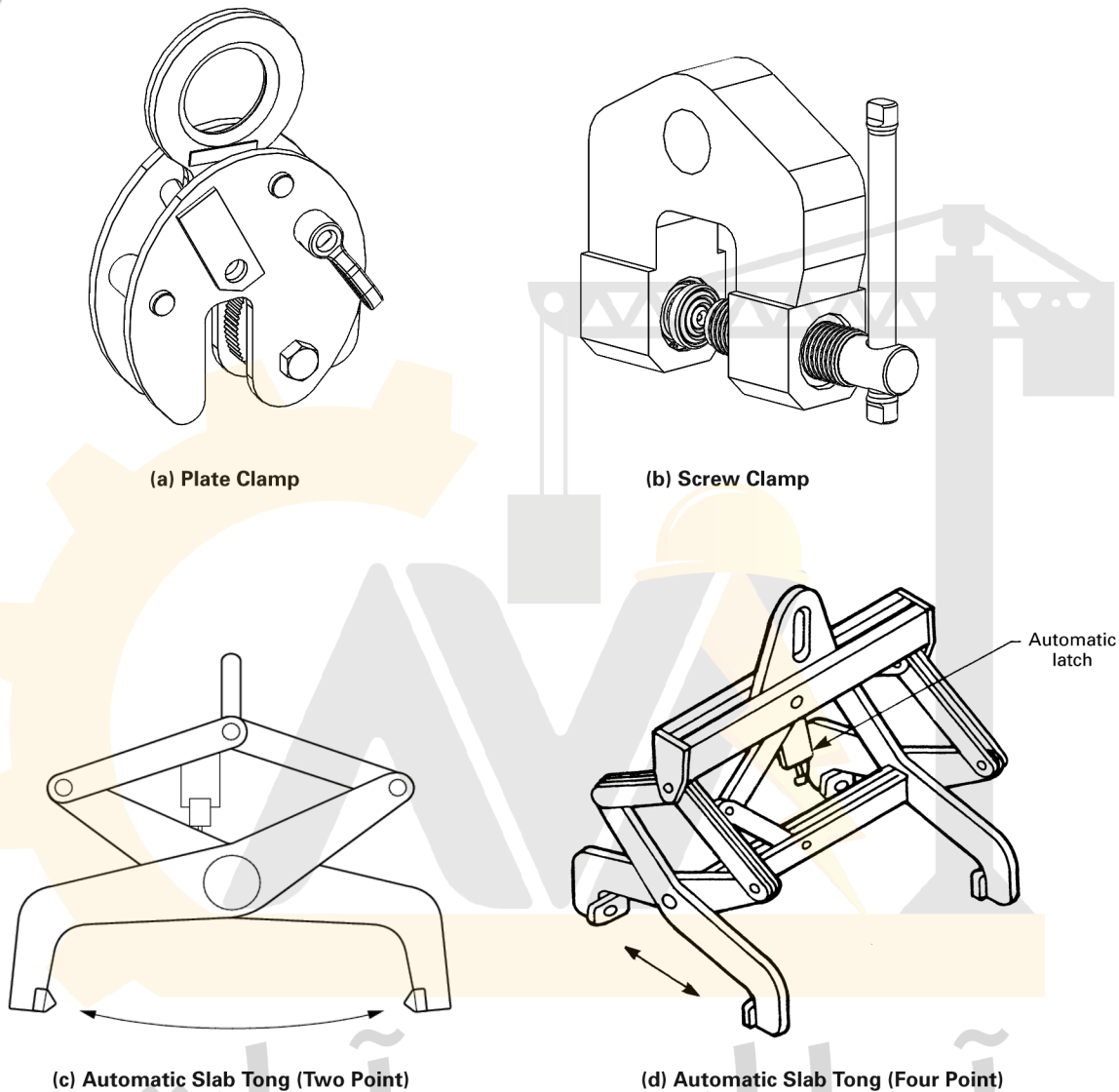
Figure 20-6.0-3 Indentation-Type Pressure-Gripping Clamps
