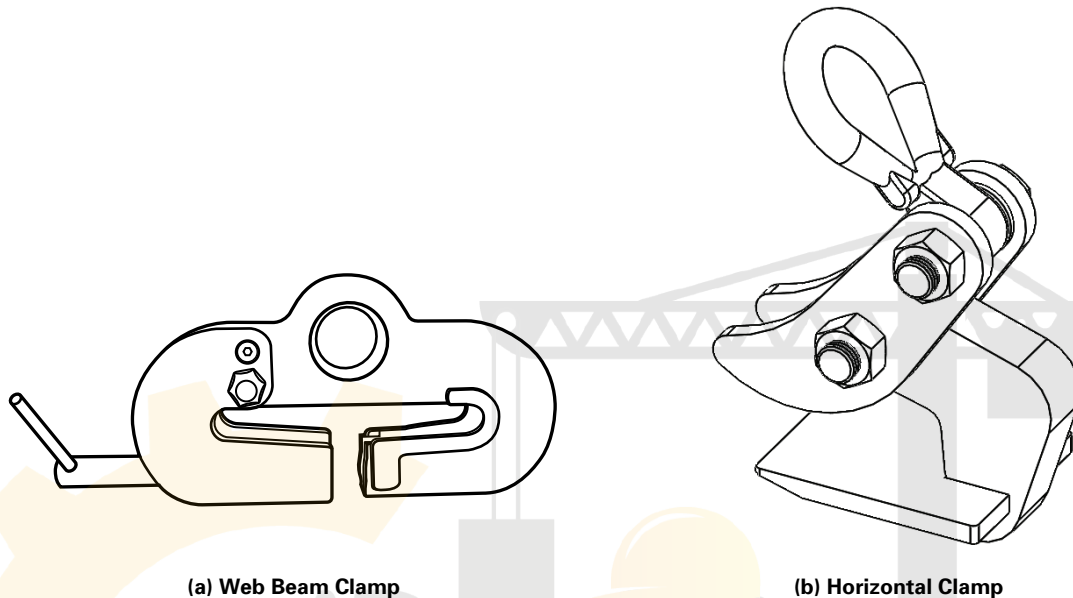
Figure 20-6.0-1 Load-Supporting Clamps
