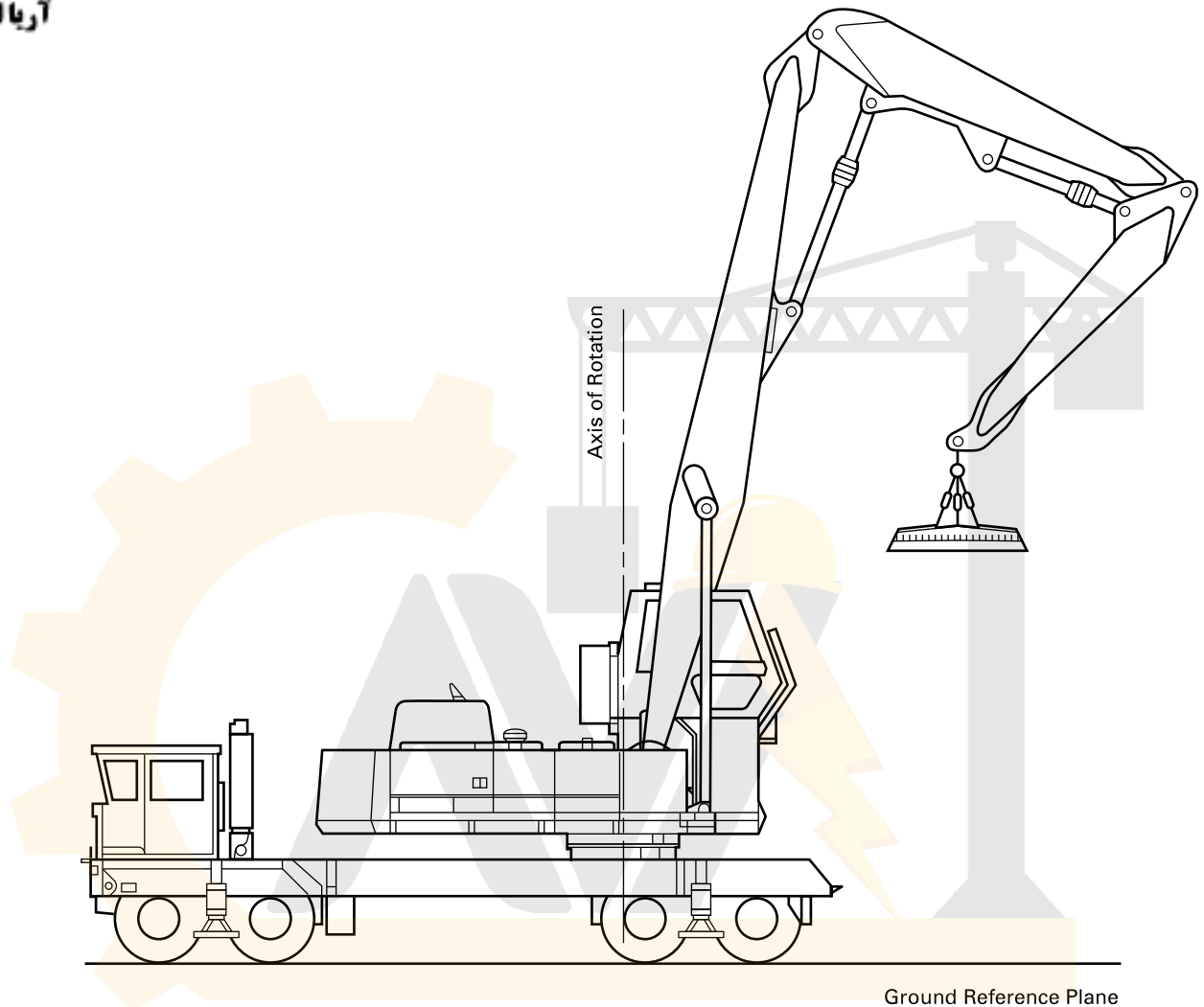
Figure 25-0.2.1-4 Wheel-Mounted Handler (Multiple Control Stations)
