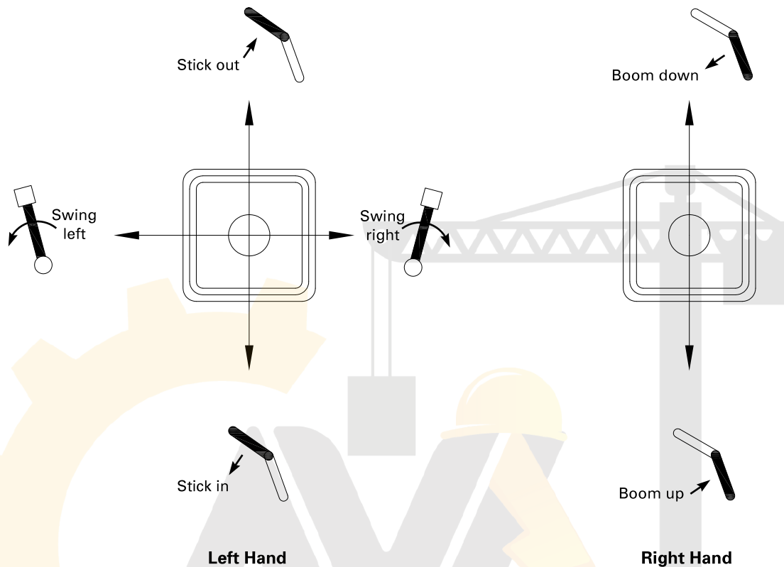
Figure 25-1.5.3-2 Primary Front Controls — Two-Piece Fronts
