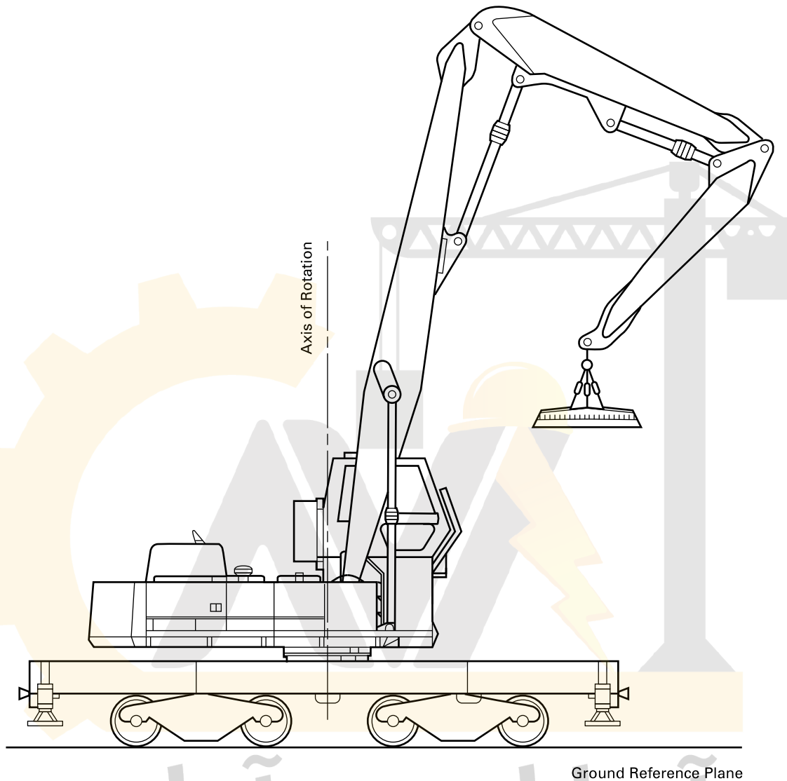
Figure 25-0.2.1-3 Rail-Mounted Handler
