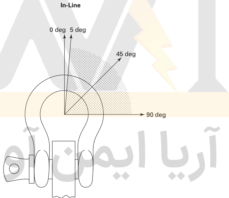
Fig. 26-1.9.4-2 Side Loading
