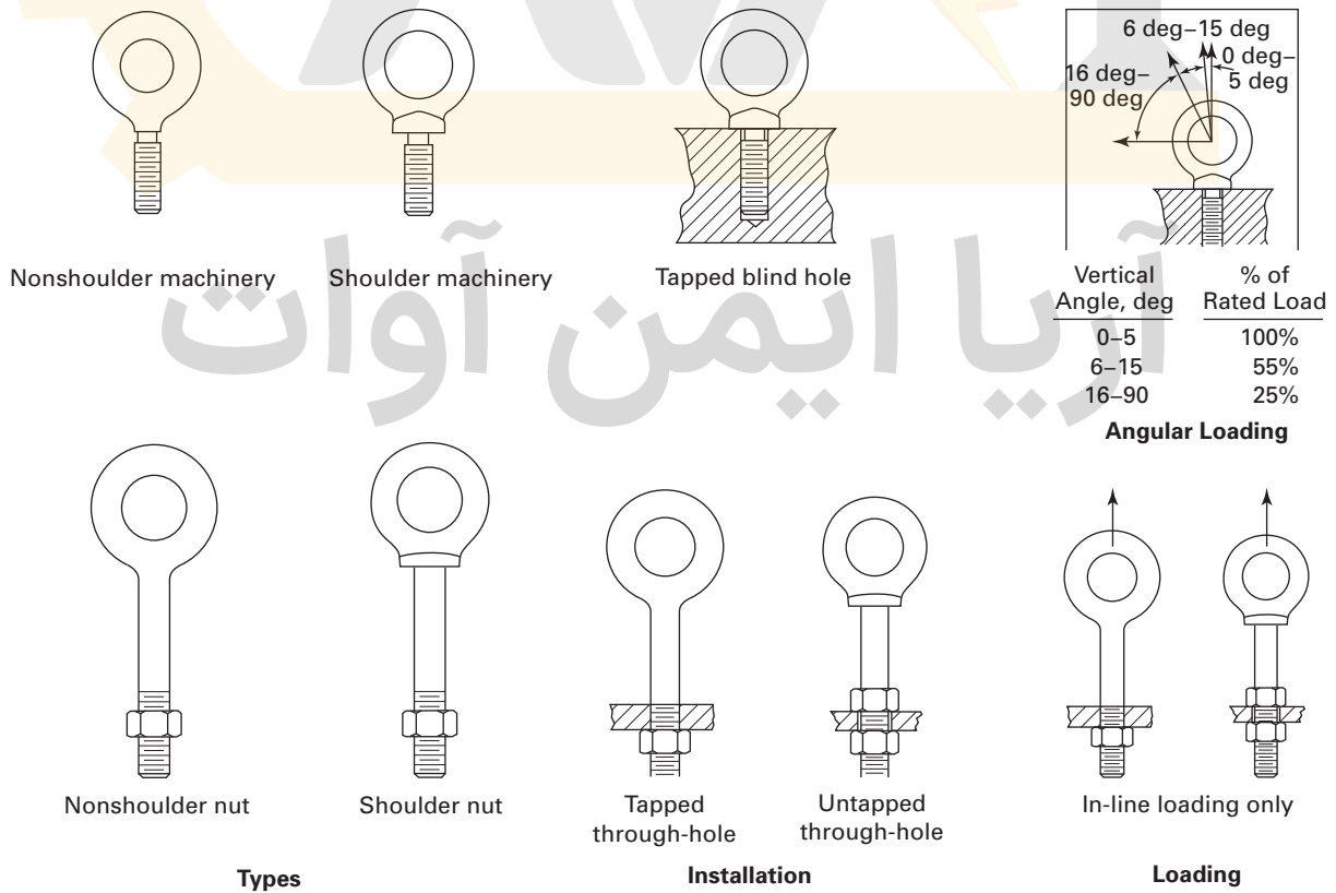
Fig. 26-2.1.1-2 Eyebolts
