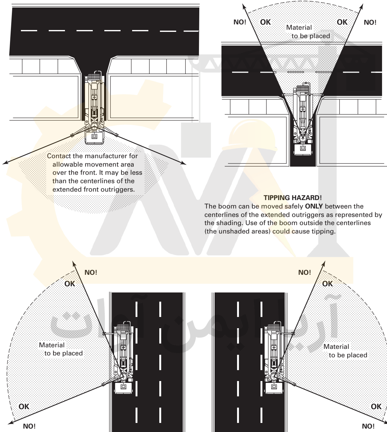
Fig. 27-3.1.5-1 Area of Extended Outriggers
