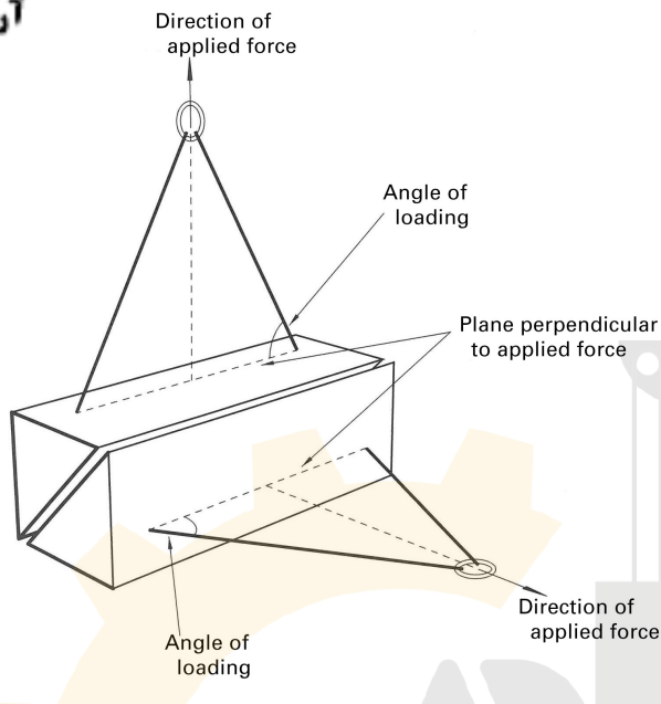
Figure 9-7.5-1 Angle of Loading
