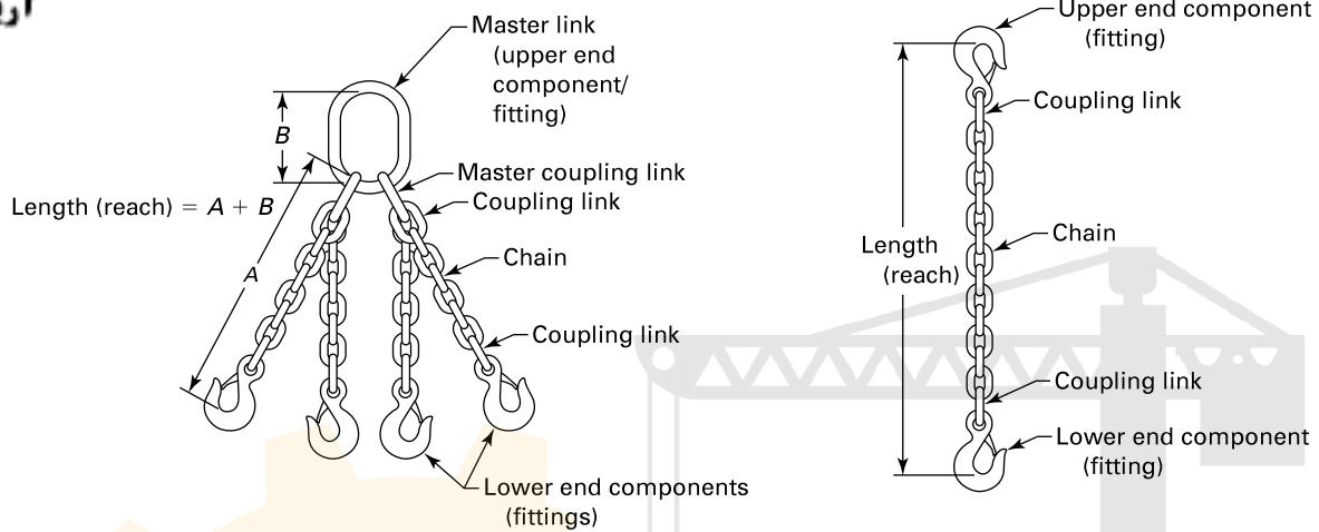
(a) Quadruple-Leg Bridle Sling Components
