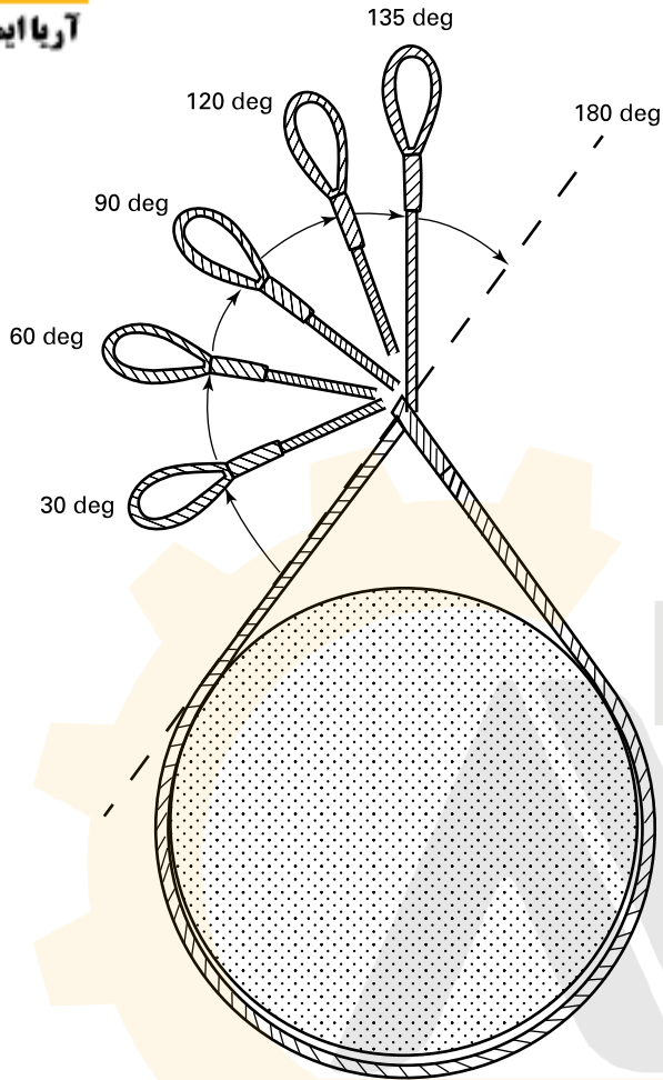
I-1 Angle of Choke: Synthetic Rope Slings
