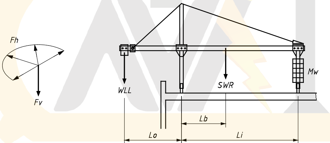
Figure 15 — Typical suspension beam
