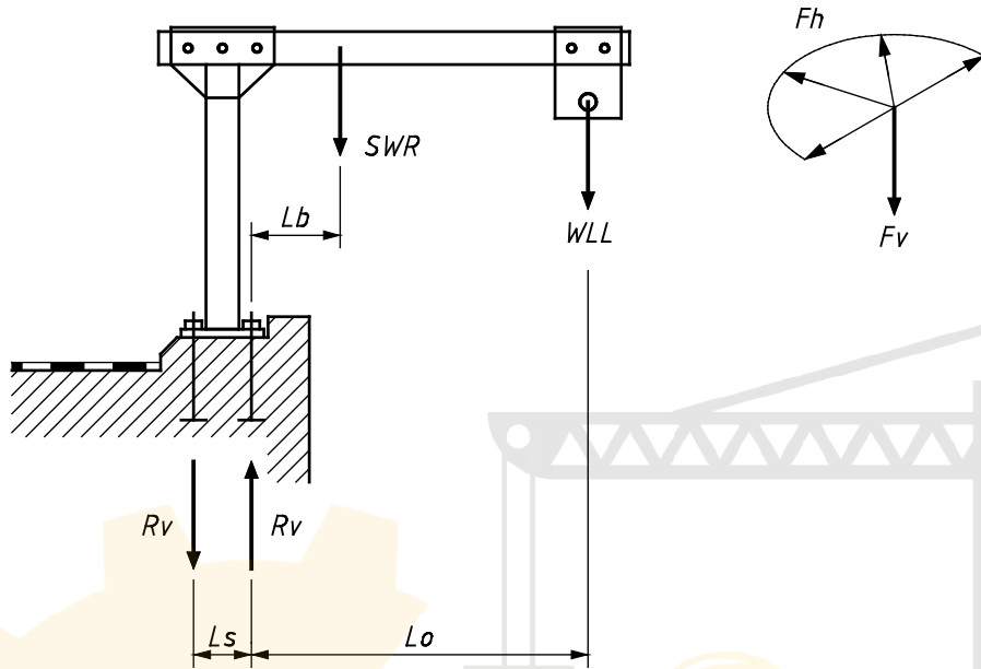
Figure 12 — Fixed Davit
