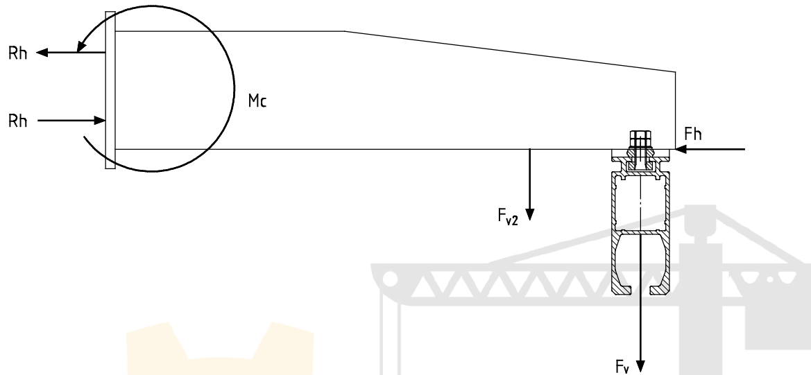
Figure D.2 — Cantilever suspension rig
