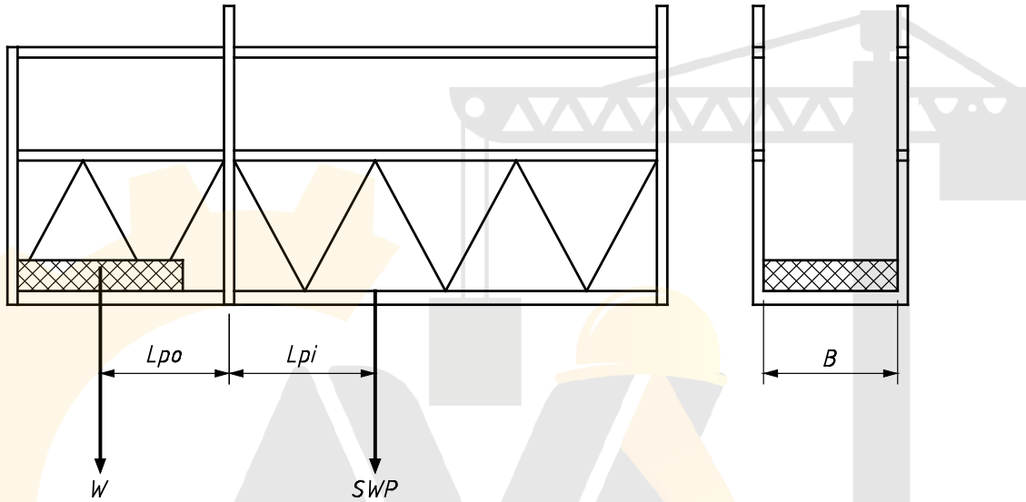
Figure 6 — Cantilevered platform
