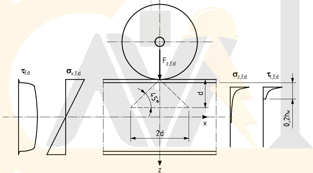
Figure G.4 — Local stresses due to wheel loads
