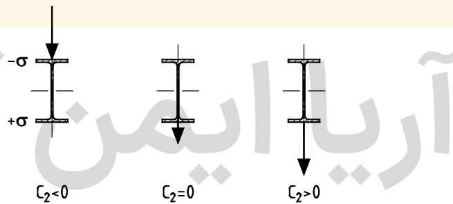
Figure G.13 — Sign of coefficient C_2
