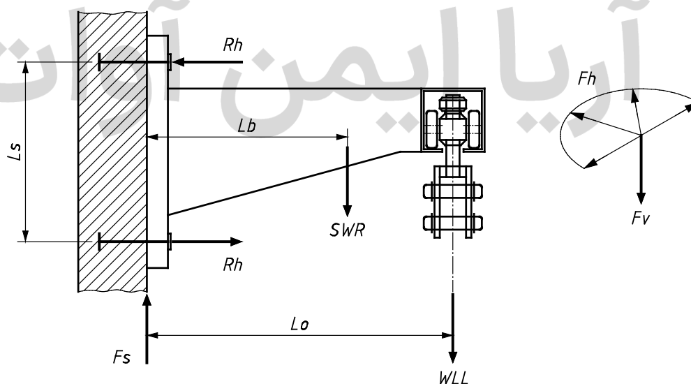
Figure 14 — Monorail
