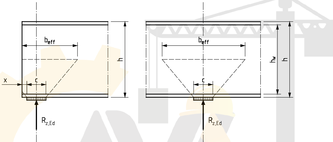
Figure G.6 — Effective width above supports
