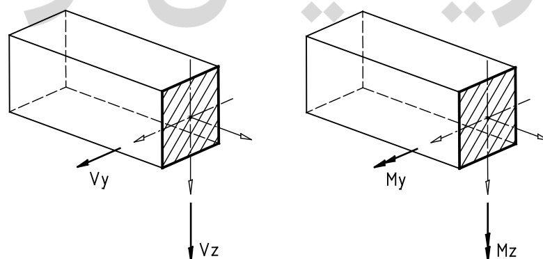
Figure G.1 — Cross-section forces
