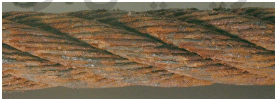
Figure H.3 — Surface of wire now greatly affected by oxidation — Rating: 60 % towards discard
